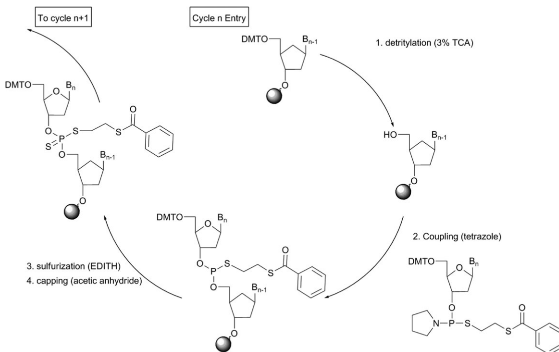
Scheme 19 A cycle of solid-phase synthesis of PS2-ODN.
